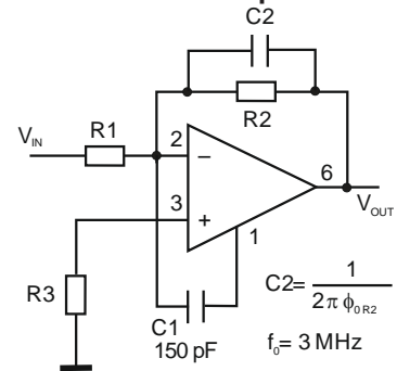
Feedforward Compensation
